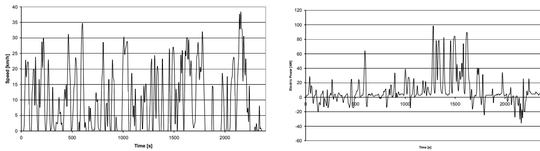
Figure 11 – Speed evolution and consumed electric power - Oreos 55 H (Lisbon - November 2001)
