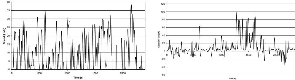
Figure 11 – Speed evolution and consumed electric power by Oreos 55 H
